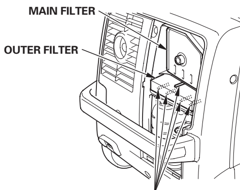
RIBS
