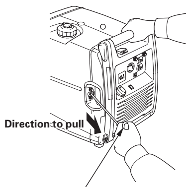
STARTER GRIP
